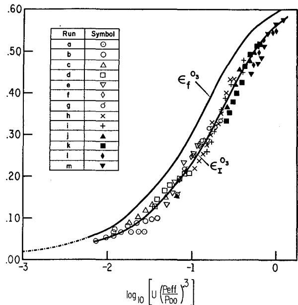
FIG. 30. Slab and column absorptivity of 9.6\text{-}\mu band of O_3 . Run means the run of experiments by Walshaw (1957). Bandwidth is assumed to be 138\text{ cm}^{-1} .
