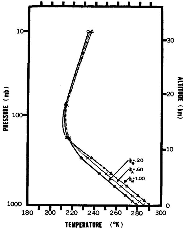
FIG. 11. Vertical distributions of radiative convective equilibrium temperature for various distributions of relative humidity.
