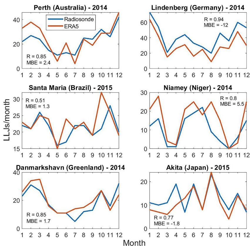
Figure 2. Validation of LLJ profiles occurrence frequency in ERA5. Shown are the monthly mean number of LLJs detected with radiosondes (blue) and in ERA5 (red) at different sites. The comparison was done for the years 2014 or 2015, as stated in the title of the figures, due to the availability of radiosonde data. The selection of the sites (see Figure 1) covers different climatic conditions.
